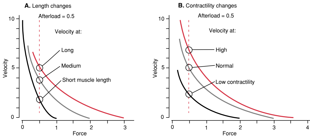
FIGURE 10.7 Effect of length and contractility changes on the force-velocity curves of cardiac muscle. A, Decreased starting length (with constant contractility) produces lower velocities of shortening at a given afterload. Because of the presence of resting force (characteristic of heart muscle), it is impos-
